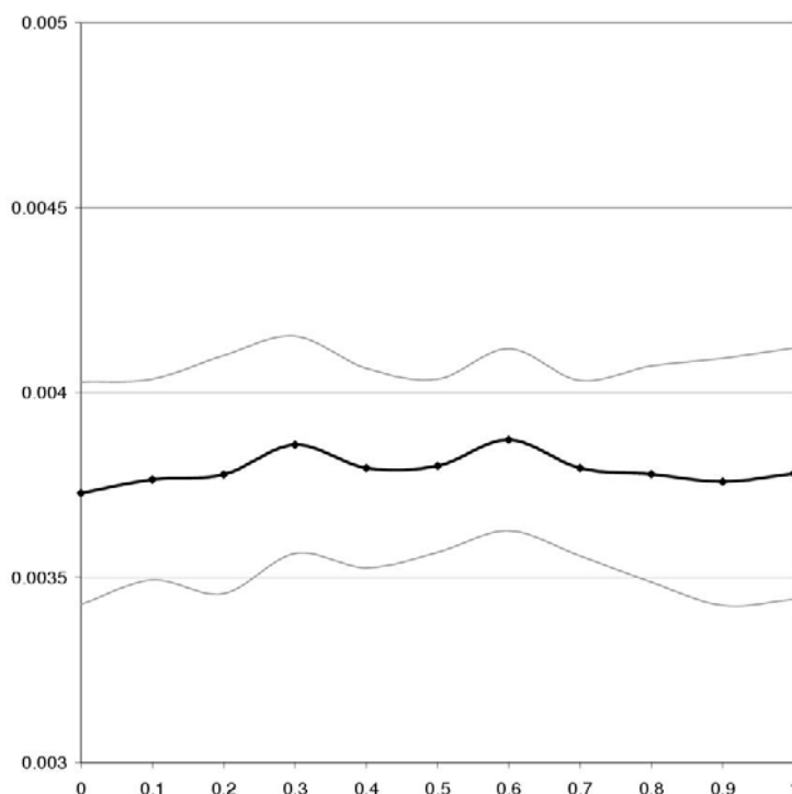
Graph of Expected Utility Earned by Each Agent as a Function of w_2 for the Equilibrium Strategy in the Scenario Described in Figure 7
